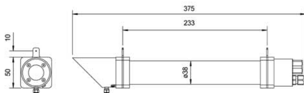
Figure 2: DR01 dimensions
