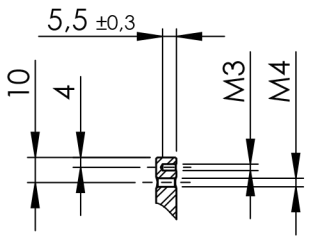
SECTION P-P
