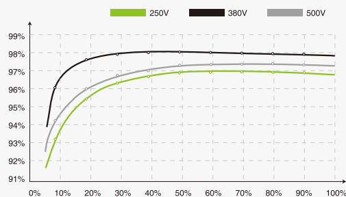
MIN 6000 TL-X efficiency
