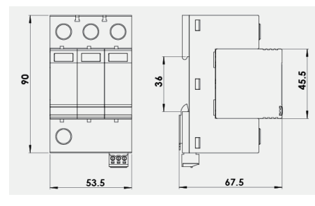
Dimension drawing
