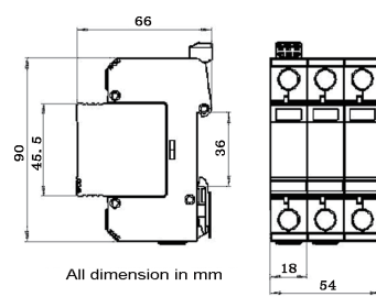
Dimension drawing
