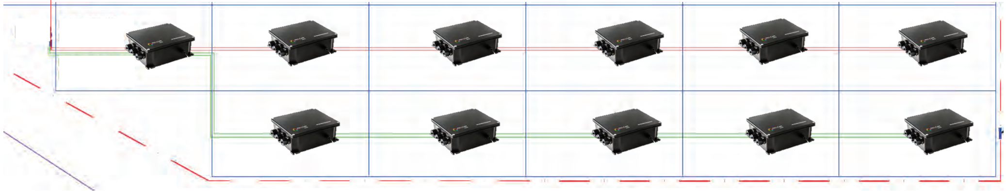
Figure 3: Cauchari I - Pry-Cam Grids on Optical Fiber Loop routing. Same arrangement on other loops
