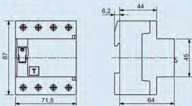
RCCB 4-pole 125 A FIP47 and FIS47
