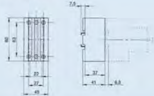
Current limiter SBMS32
