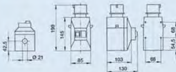
Insulated enclosure with CEE plug
