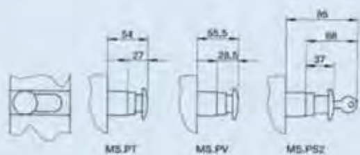
Emergency-stop button MS.PT – PS.PS2
