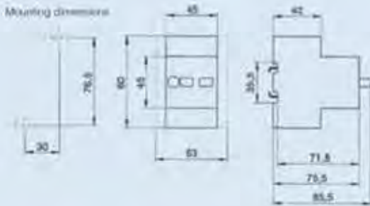
Motor protective circuit breaker MS
