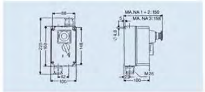
Padlocking facility for max. 3 padlocks lock bracket Ø 4 - 8 mm
