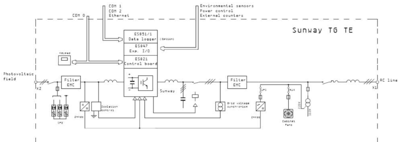
Figure 1: Block schematics
