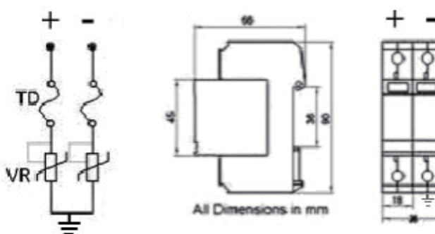
Common mode DC Surge arrester for Photovoltaic protection against surges at the boundaries from lightning protection zone OB-1 and higher.
