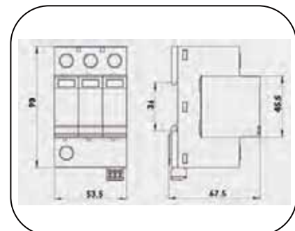
Dimension drawing
