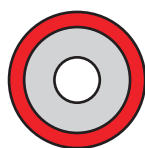
12 mm Ø Brass Insert Terminal for M5 Bolt TYPE FT 2
