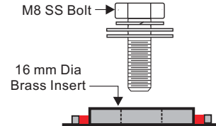
TYPICAL TRIPLE SEAL DETAIL
