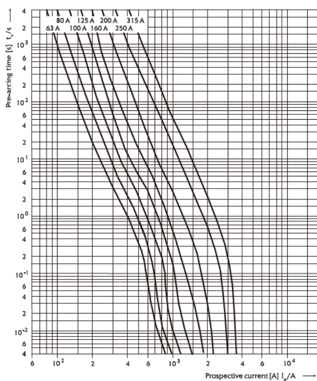
NH DC 1100V t-I characteristics
