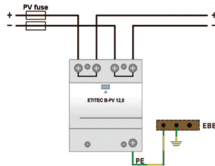
V - Connection ETITEC B-PV
