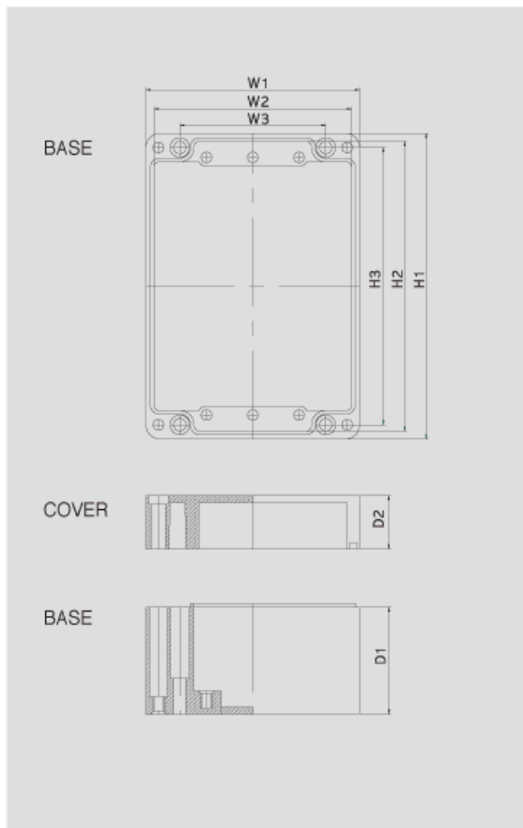
Dimension (허용오차 allowance \pm 1\text{mm} )
