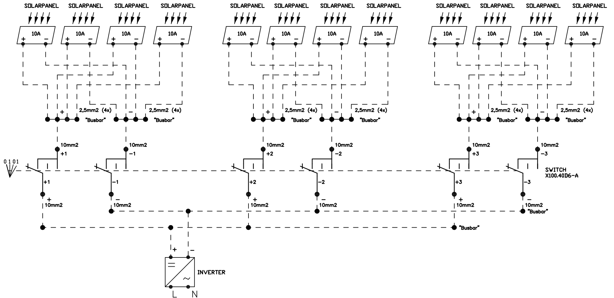
PRINCIPE SCHEME 6 POLE SWITCH (120A)
