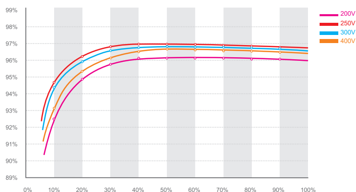
Growatt 1500-S efficiency
