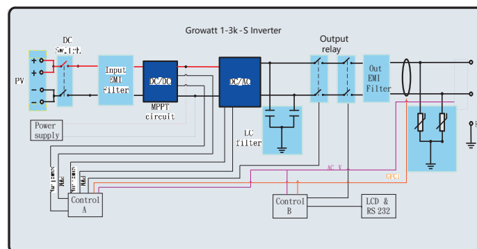
Growatt 1-3k -S topology
