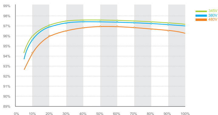
Growatt 11000tl-us efficiency
