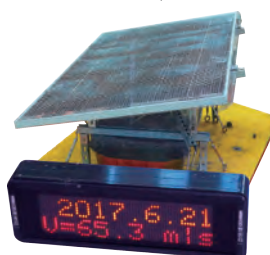
日照計/溫濕度信號傳送器/表面溫度感應器/風速風向計 Pyranometer/Outdoor temperature and humidity transmitter/ TS Surface temperature sensor/Wind speed and direction
