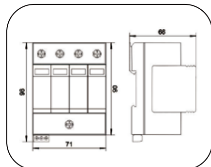
Dimension drawing
