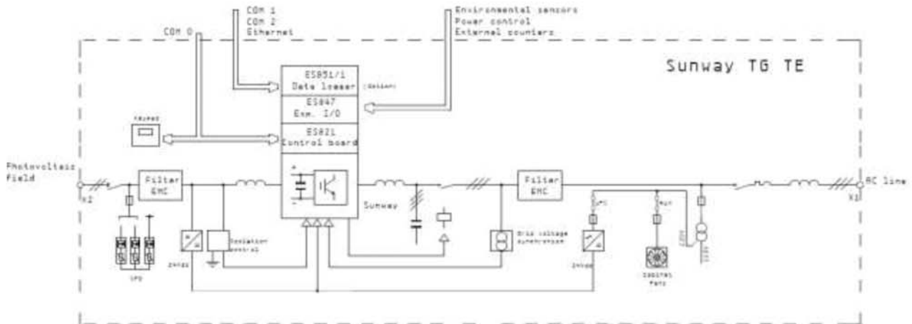
Figure 1: Block schematics
