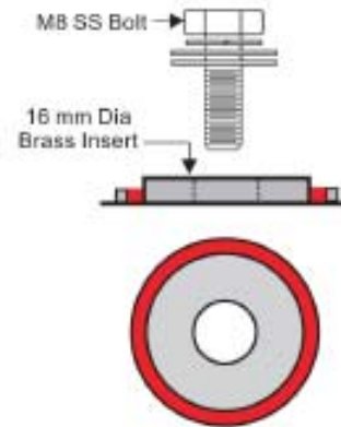
16 mm \varnothing Brass Insert Terminal for M8 Bolt
