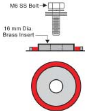
16 mm \varnothing Brass Insert Terminal for M6 Bolt
