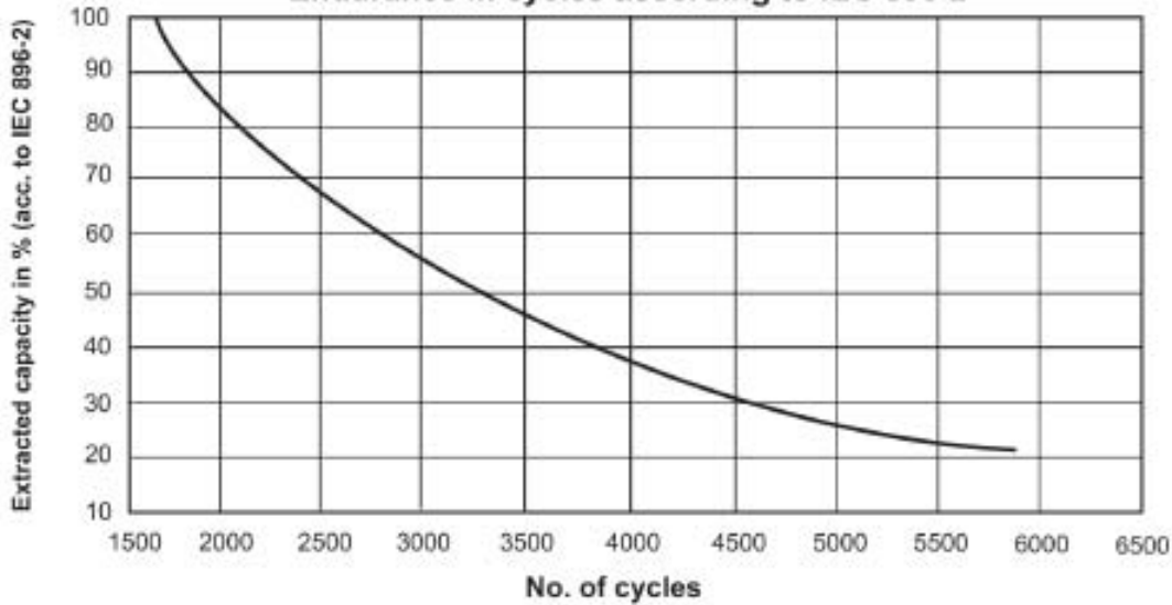
Endurance in cycles according to IEC 896-2
