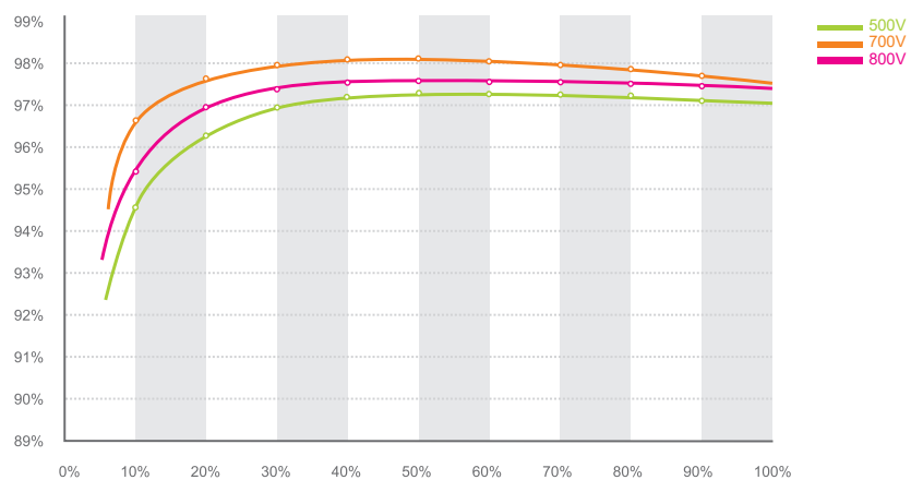
Growatt 40000 TL3 efficiency
