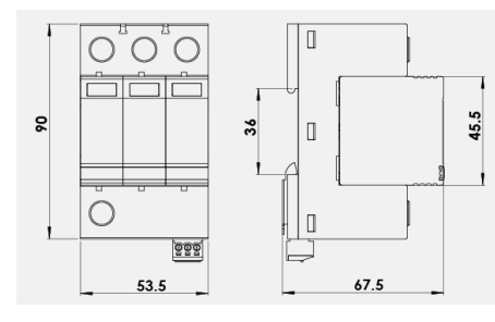
Dimension drawing
