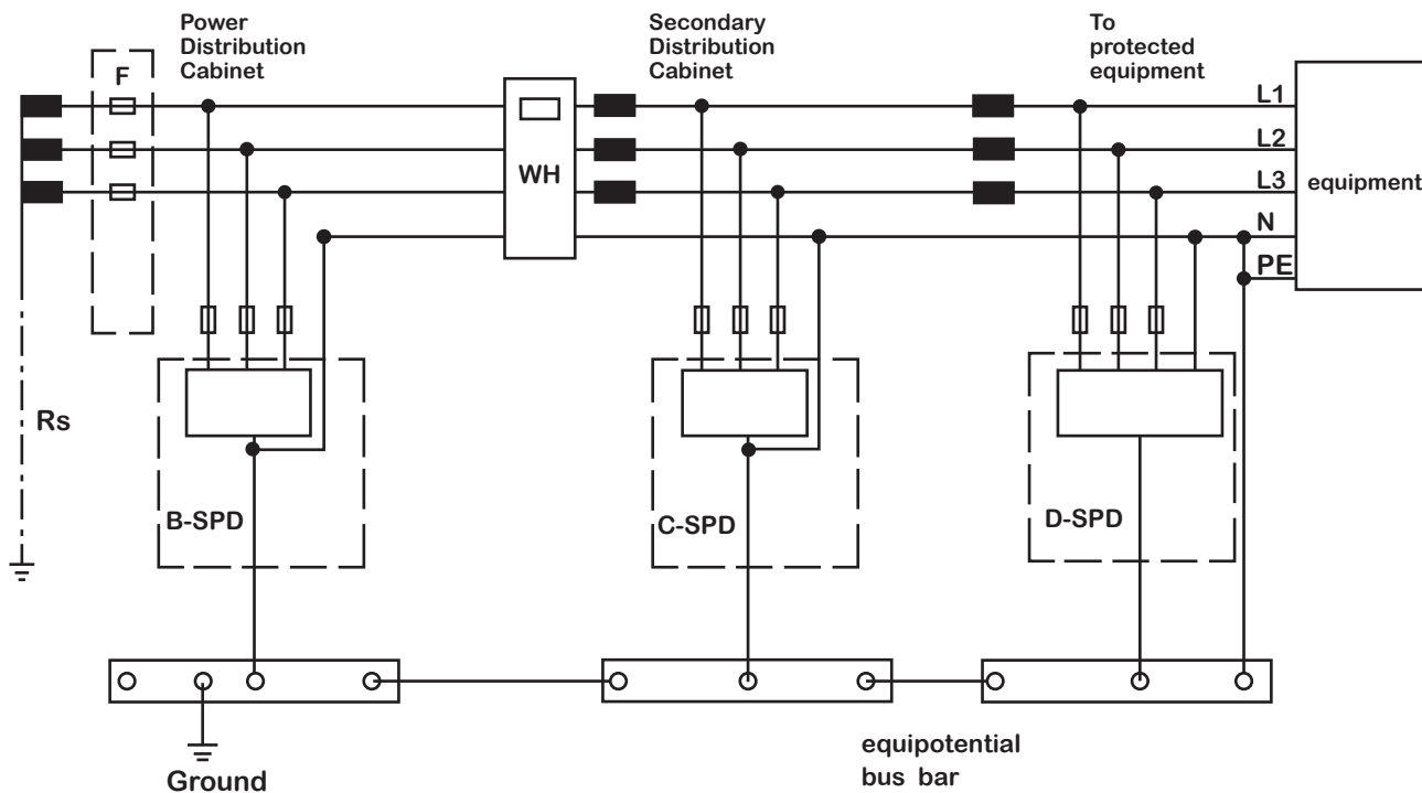
IT system
