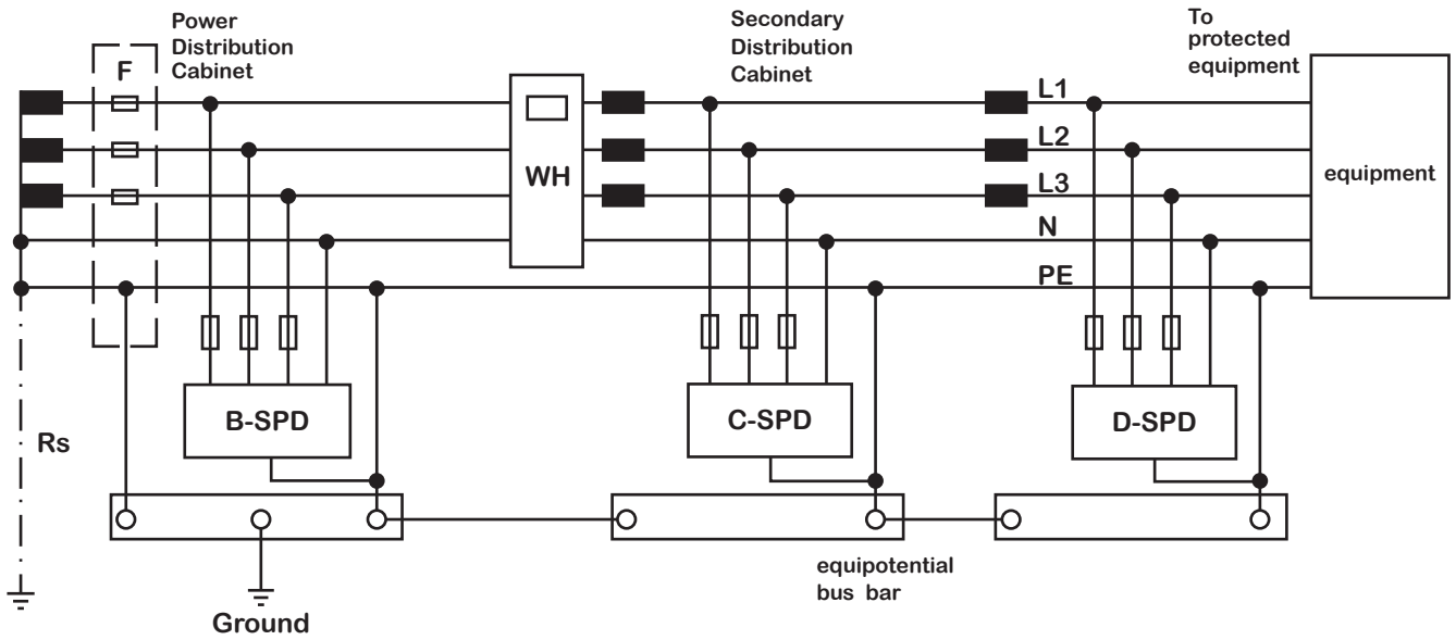
TN-S system
