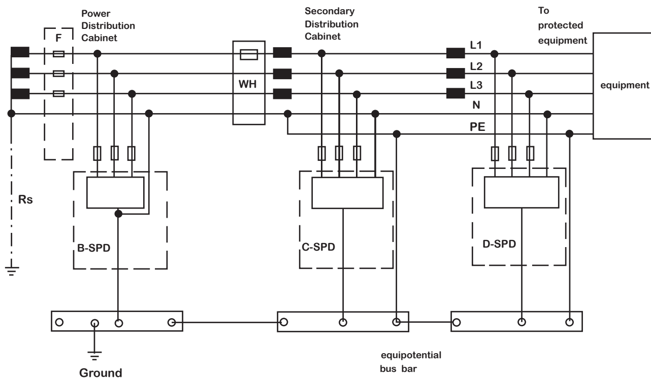
TN-C-S system
