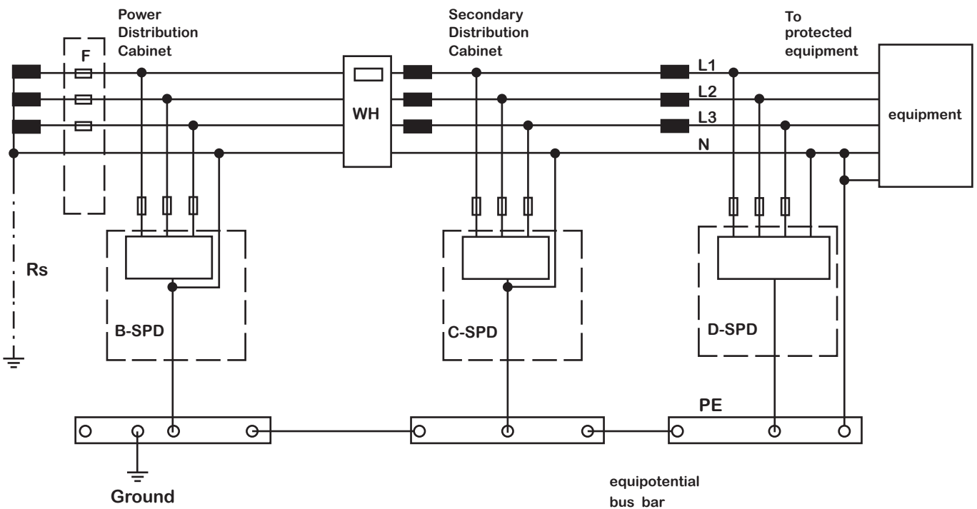
TN-C system
